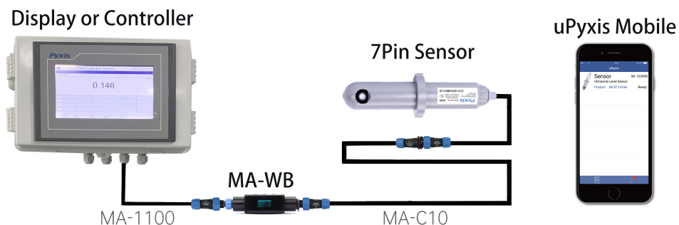
Figure 5. 7-Pin Sensor with MA-WB and uPyxis Mobile
